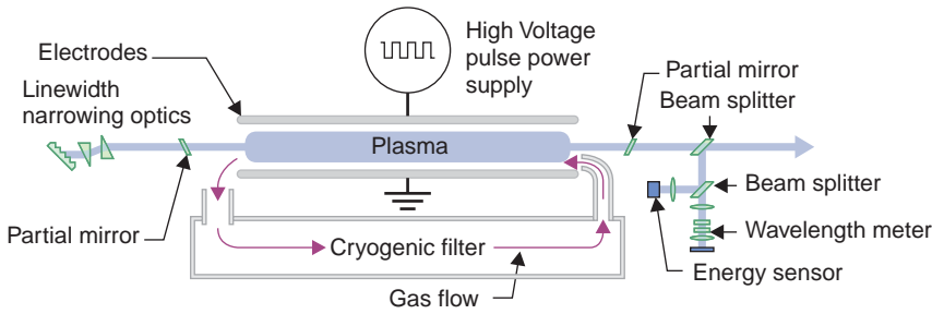
Excimer laser light source
